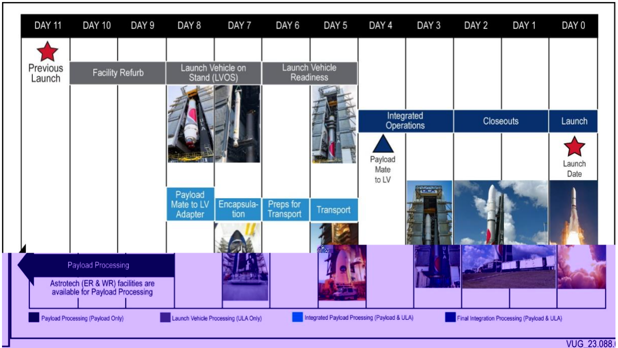
Figure 5.3-1 Baseline SLC-41 Single Launch Flow
