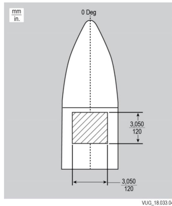
Figure 4.3.4-1 Customer Logo Location
