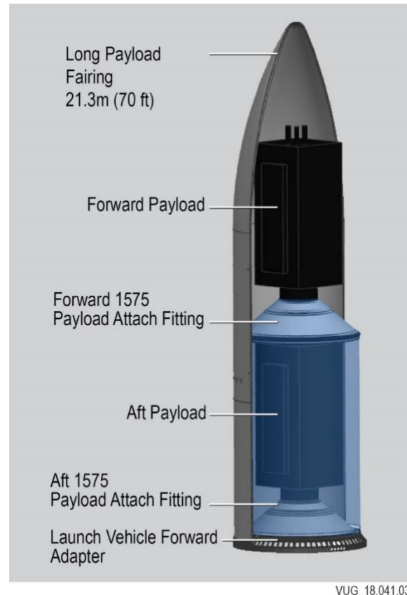
Figure 4.6.1-1 Multi-Launch System
