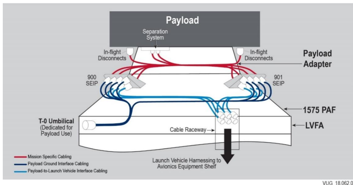
Figure 4.4-1 Payload-to-Launch Vehicle Electrical Interfaces Overview
