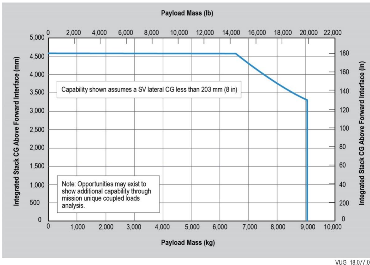
Figure 4.2.1.1-3 1575 PAF Structural Capability
