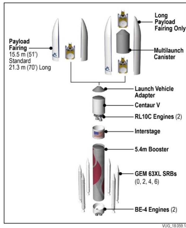
Figure 1.4-1 Vulcan Centaur Launch Vehicle Configurations
