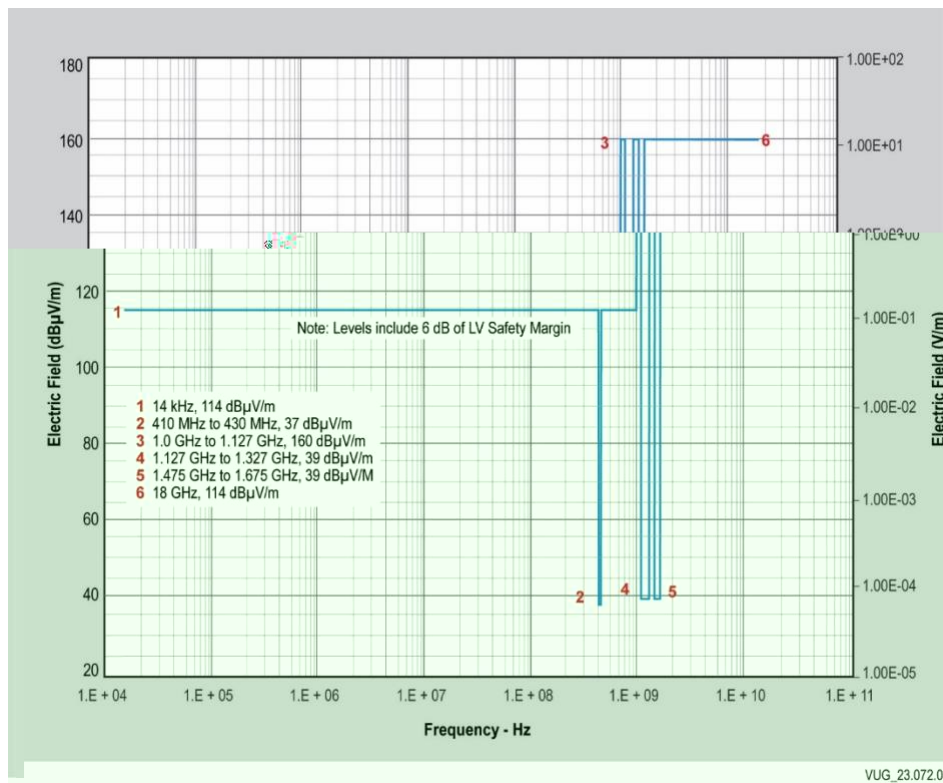
Figure 3.1.2.2-1 Maximum Payload Radiated Emissions
