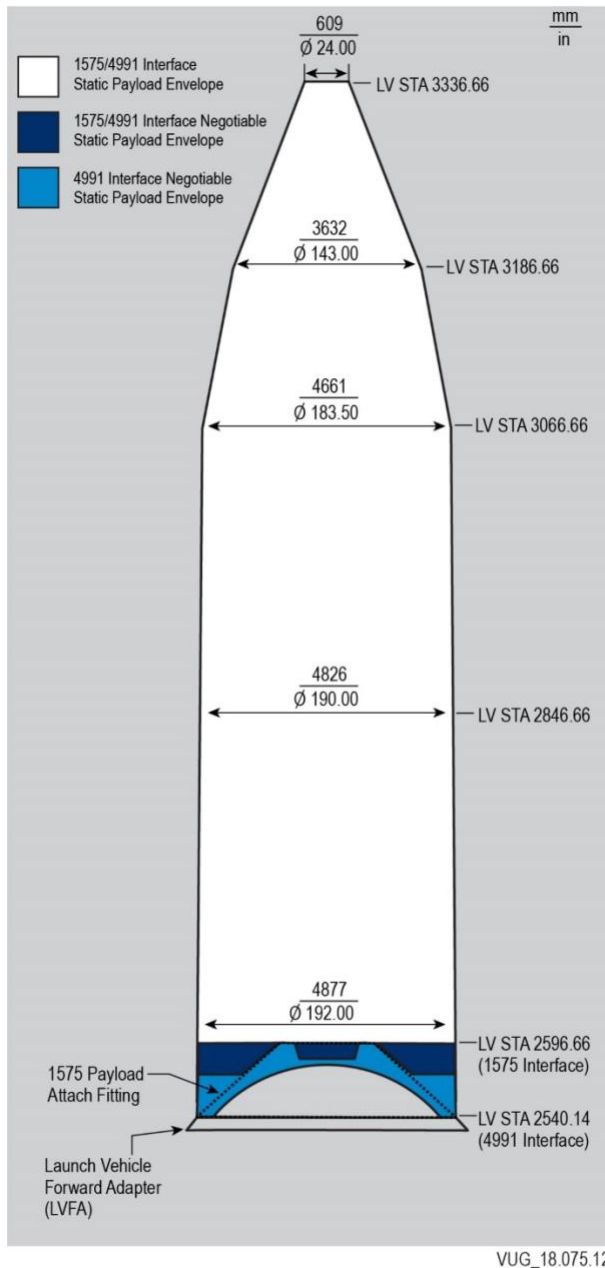
Figure 4.3.1-2 Vulcan Centaur 21.3-m (70-ft.) PLF Simplified Static Payload Envelope
